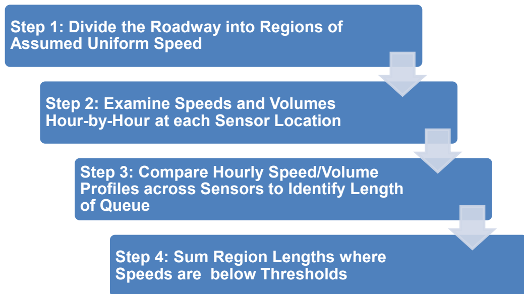
Figure 3-8. Steps to Estimate Queue Lengths from Spot Speed Sensor Data
